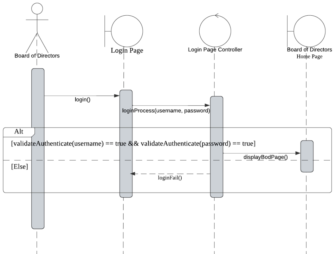
Figure x : Sequence Diagram for Board of Directors Login Process
