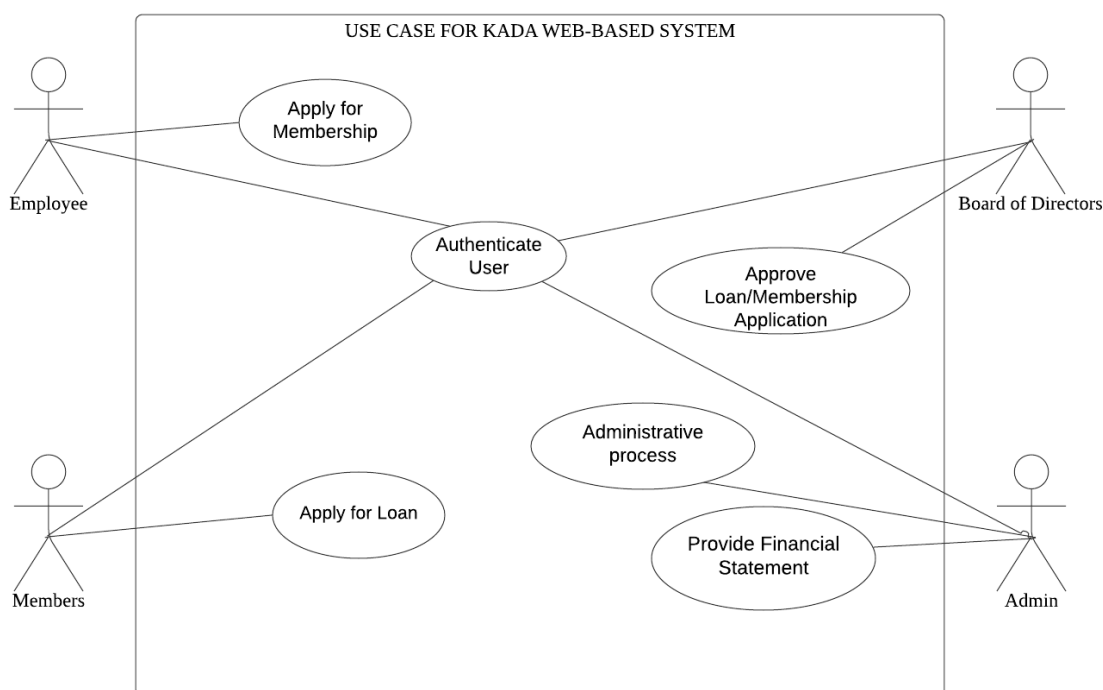
Figure 2.1: Use Case Diagram for KADA's Cooperative Web-Based System
