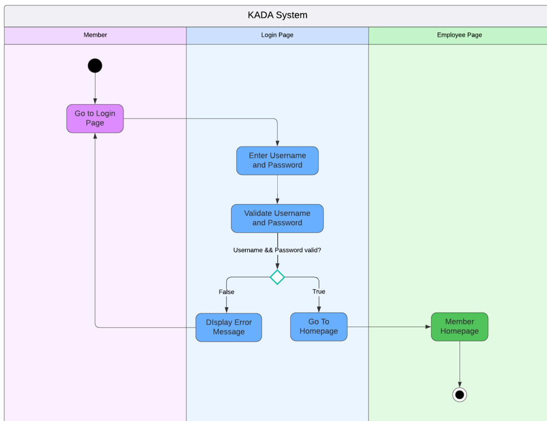
Figure x : Activity Diagram for Member Login Process
