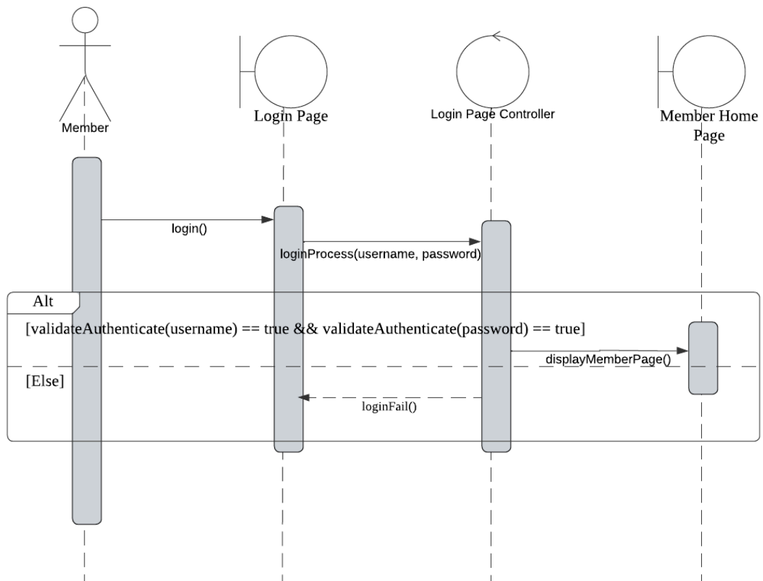
Figure x : Sequence Diagram for Member Login Process
