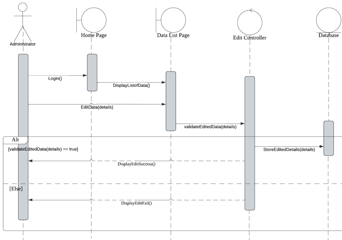
Figure x : Sequence Diagram for Administrative Process for Editing Data/Record
