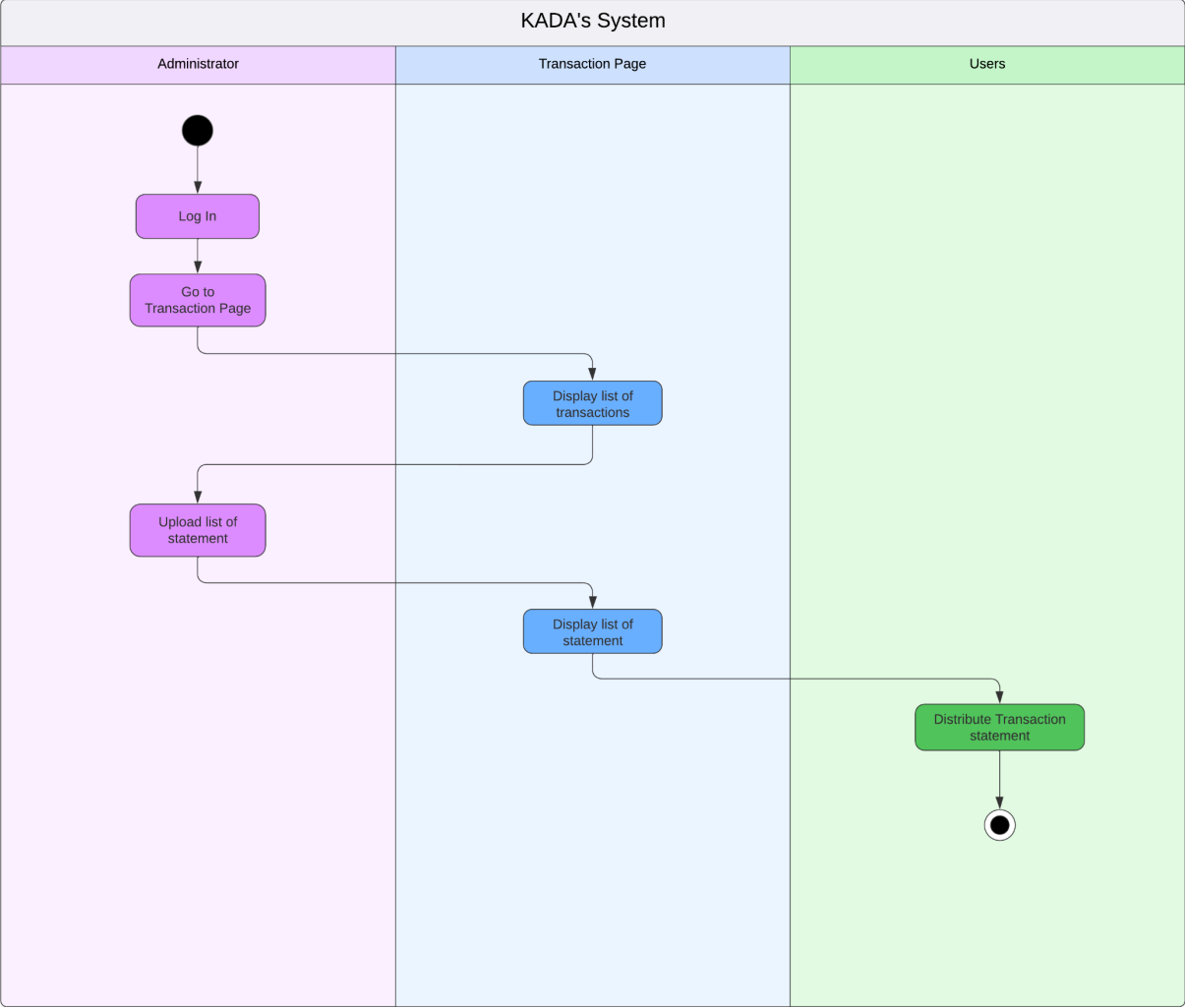
Figure x : Activity Diagram for Administrator to Provide Financial Statement Process
