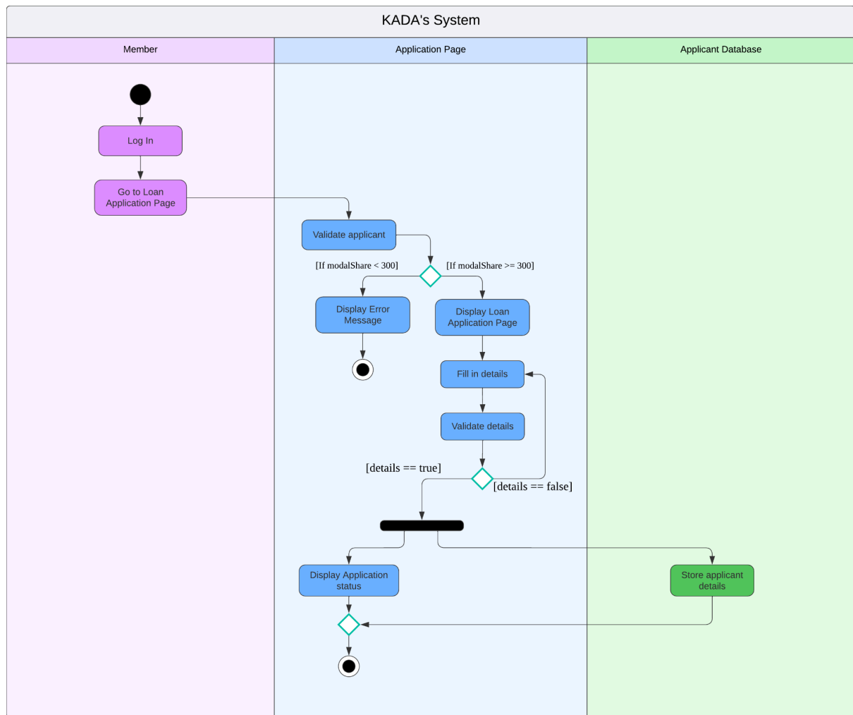
Figure x : Activity Diagram for Member to Apply Loan Process
