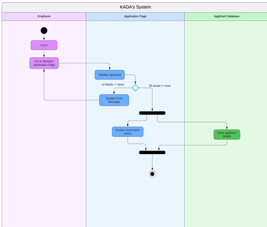
Figure x : Activity Diagram for Applying Membership Process
