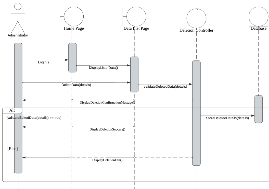
Figure x : Sequence Diagram for Administrative Process for Deleting Data/Record
