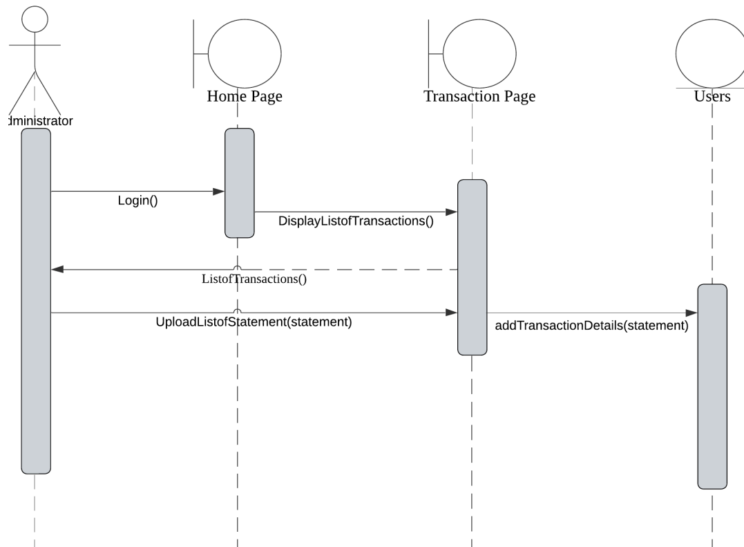
Figure x : Sequence Diagram for Administrator to Provide Financial Statement Process
