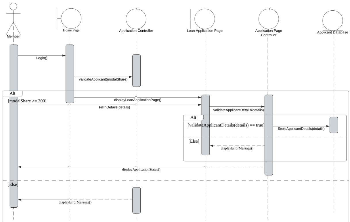
Figure x : Sequence Diagram for Member to Apply loan Process
