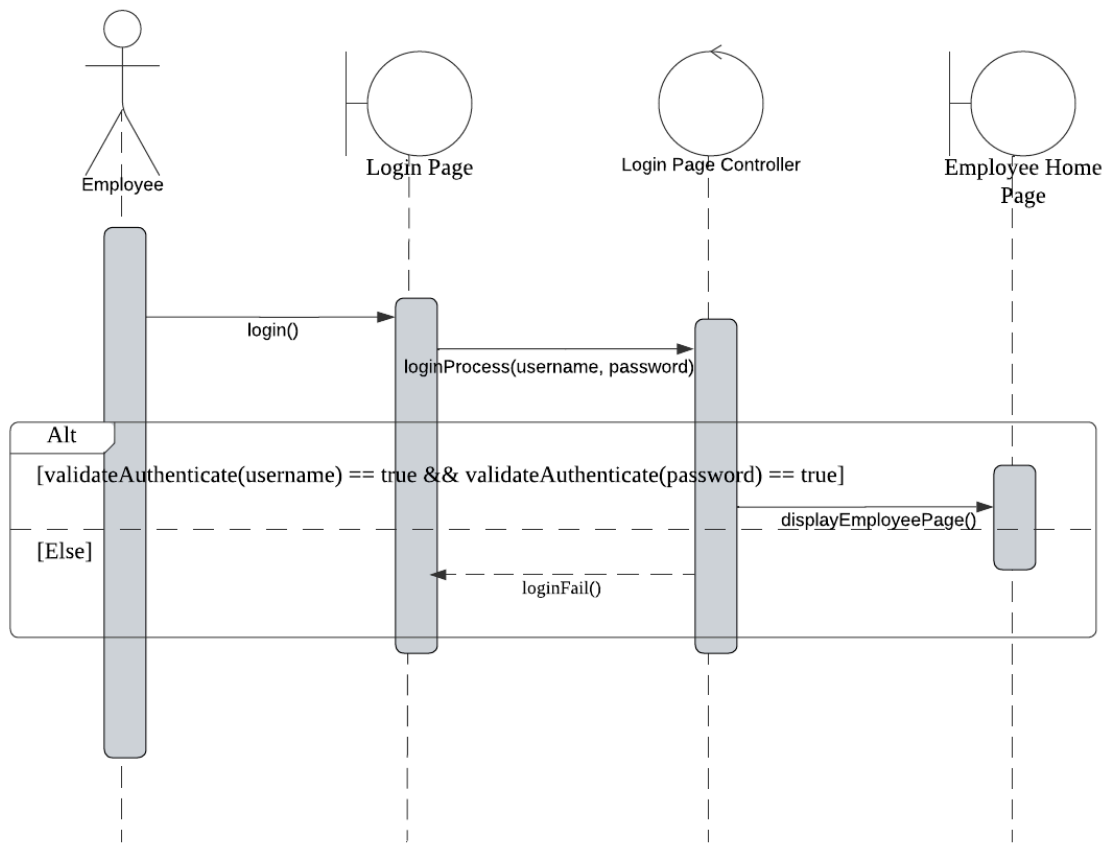
Figure x : Sequence Diagram for Employee Login Process
