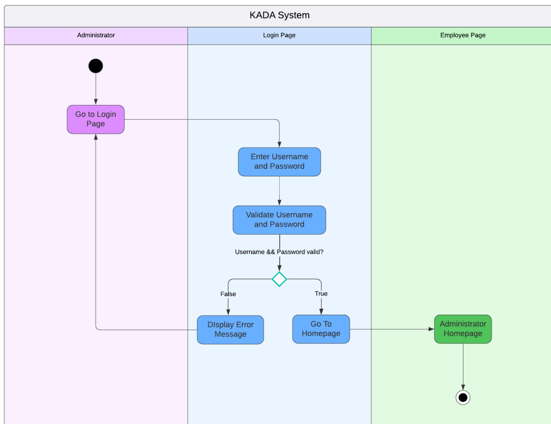
Figure x : Activity Diagram for Administrator Login Process
