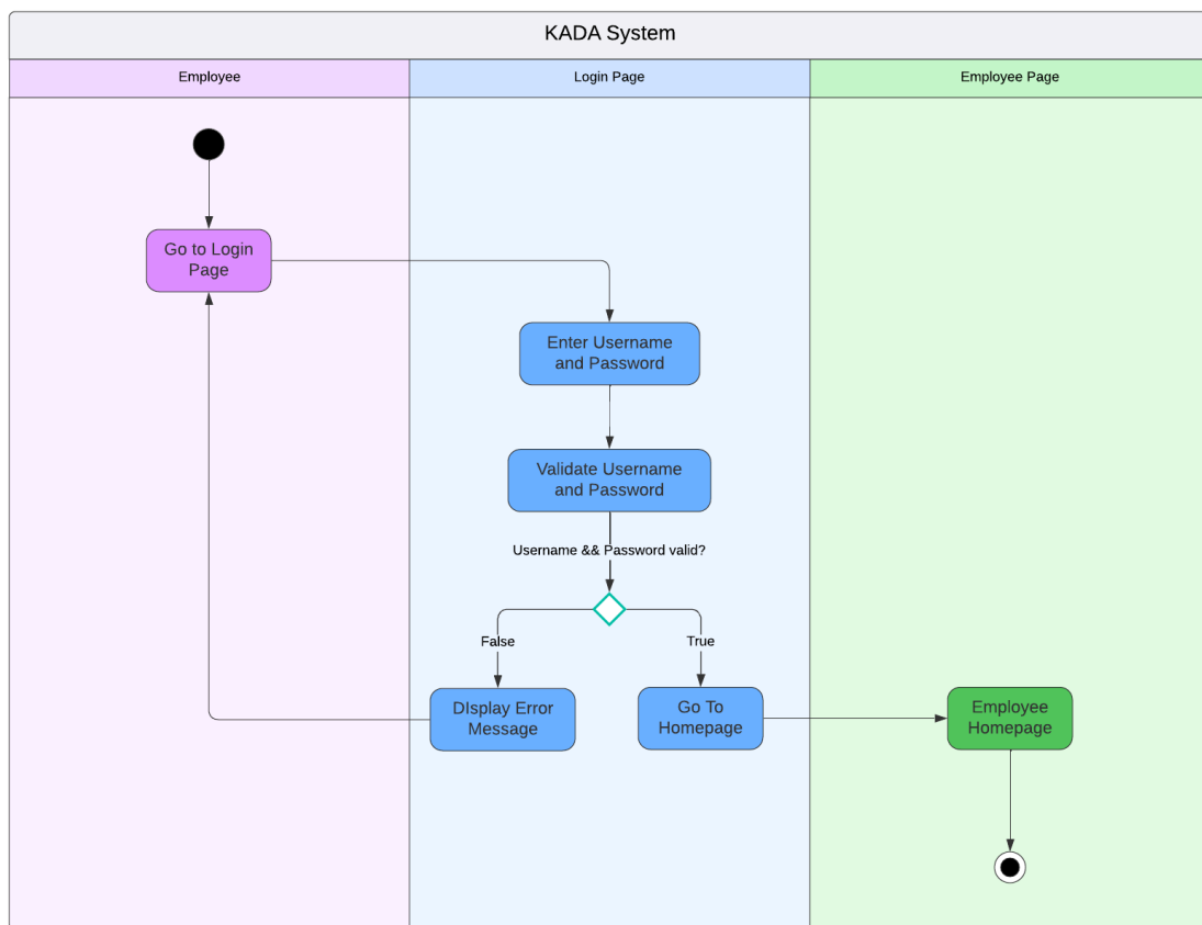
Figure x : Activity Diagram for Employee Login Process
