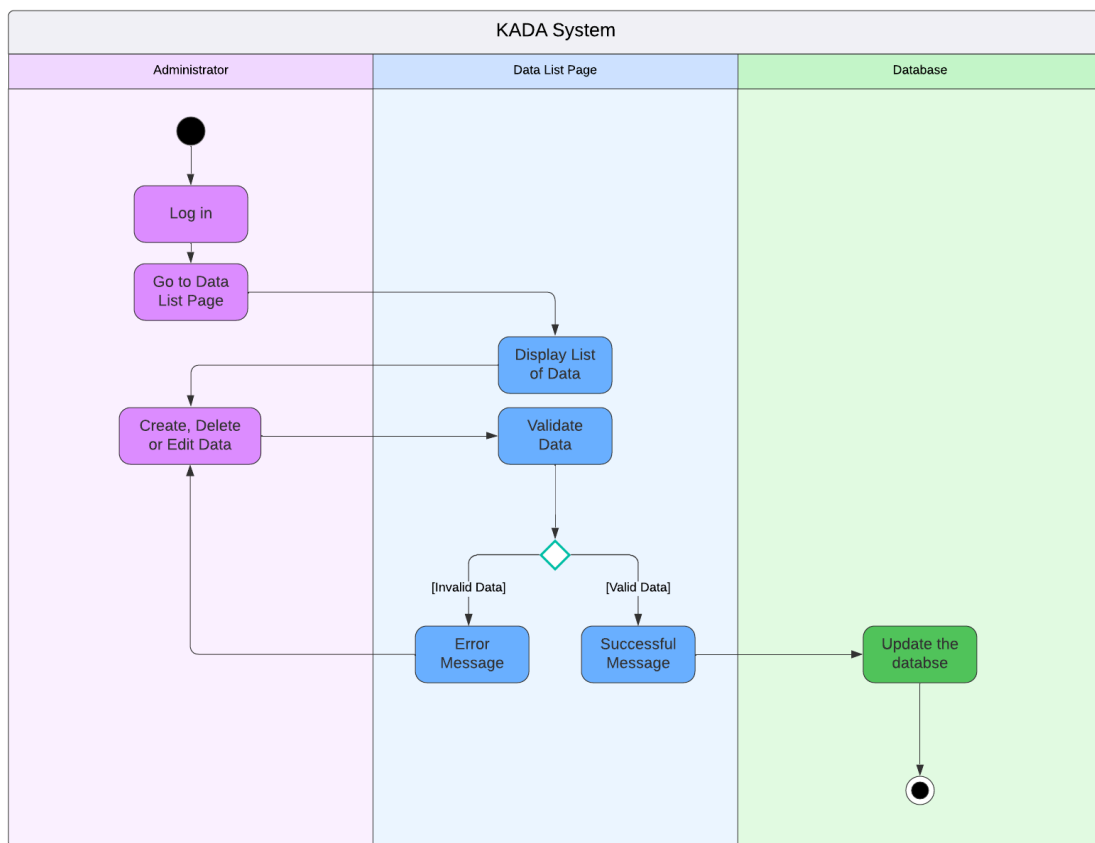
Figure x : Activity Diagram for Administrator doing Administrative Process
