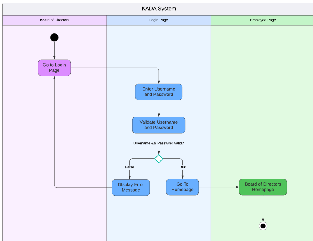
Figure x : Activity Diagram for Board of Directors Login Process
