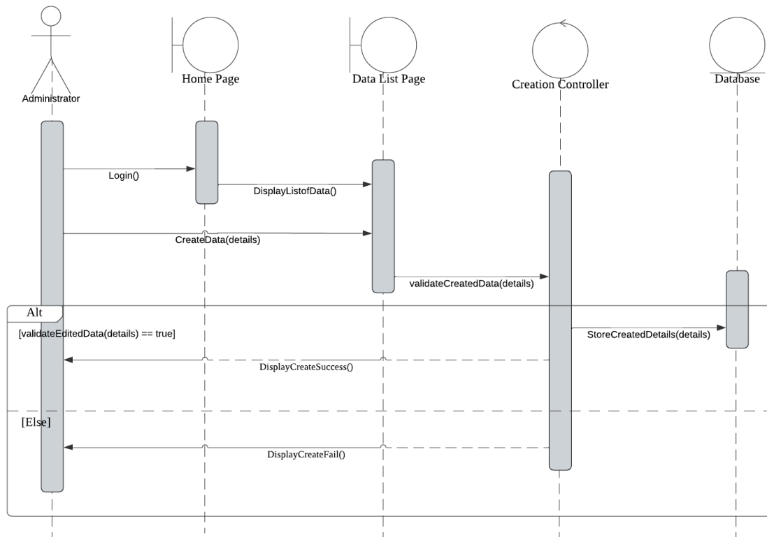
Figure x : Sequence Diagram for Administrative Process for Creating New Data/Record
