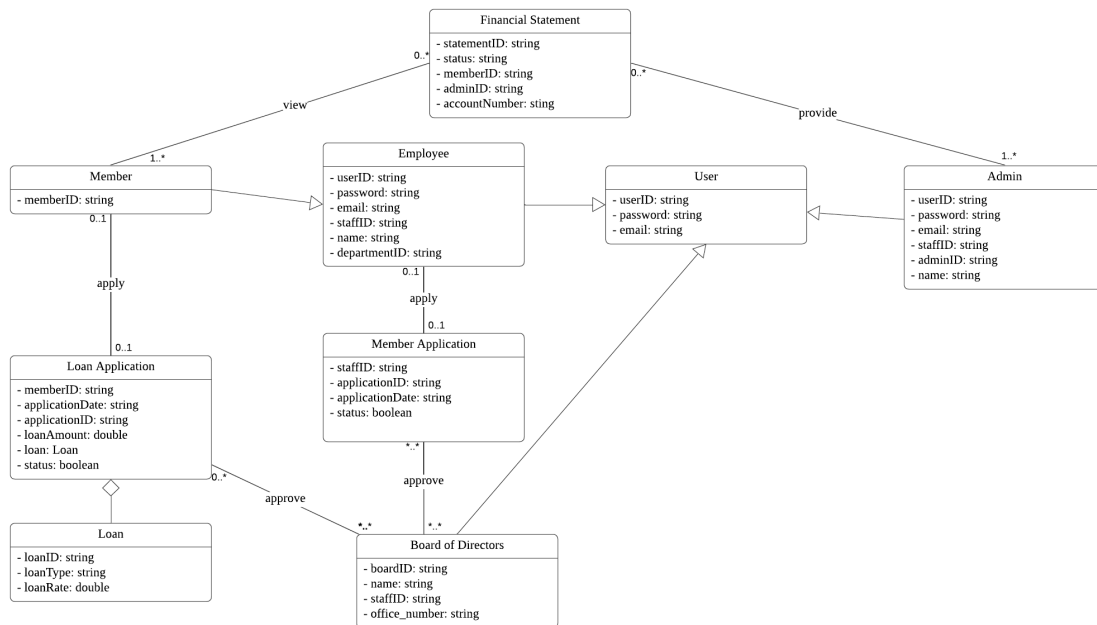
Figure 2.2: Domain Model for KADA's Cooperative Web-Based System
