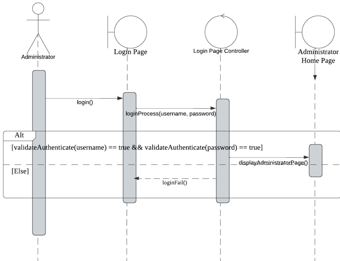
Figure x : Sequence Diagram for Administrator Login Process
